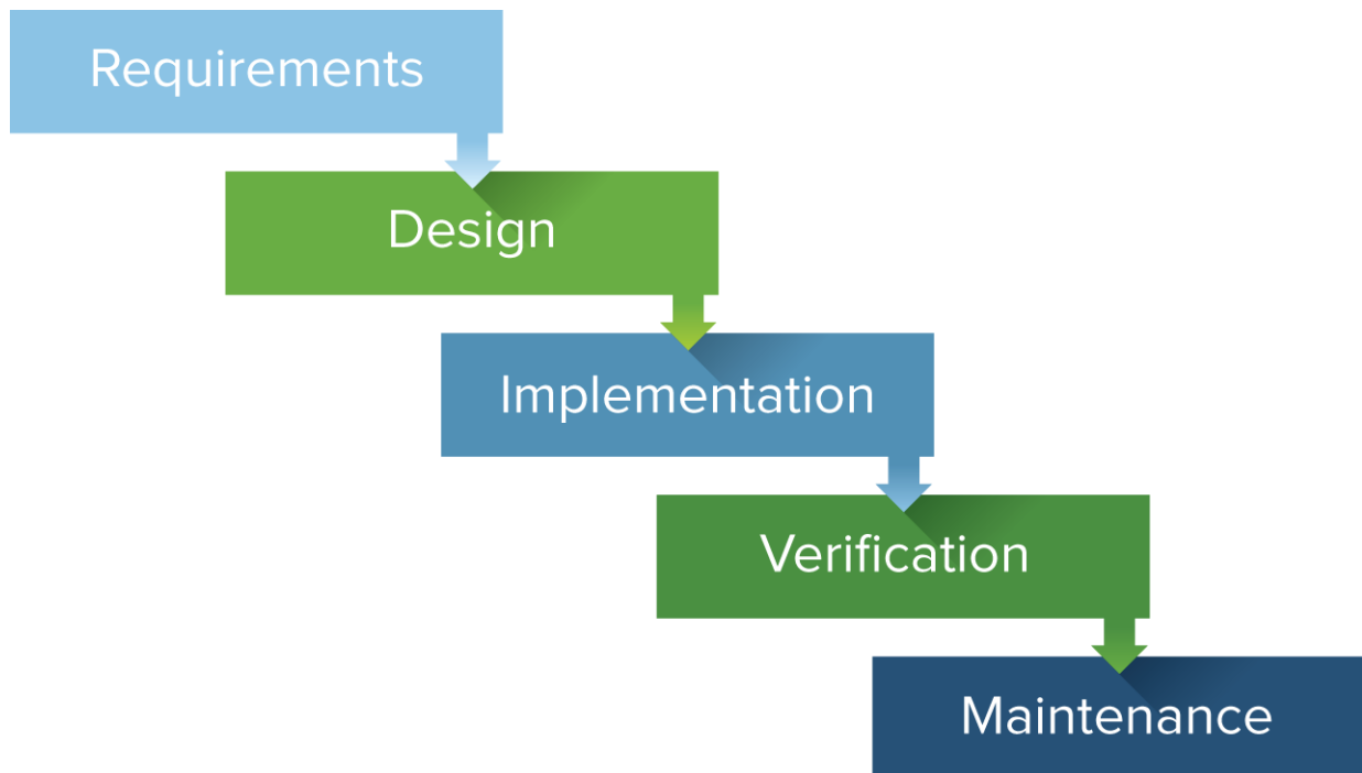
Image1- Waterfall model
